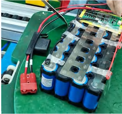
Inner structure
